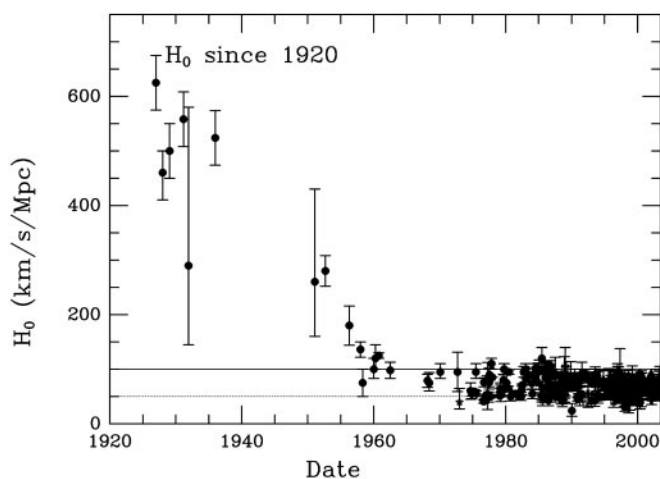
Fig. 2. Published values of the Hubble constant vs. time. Revisions in Hubble's original distance scale account for significant changes in the Hubble constant from 1920 to the present as compiled by John Huchra of the Harvard-Smithsonian Center for Astrophysics. At each epoch, the estimated error in the Hubble constant is small compared with the subsequent changes in its value. This result is a symptom of underestimated systematic errors.
