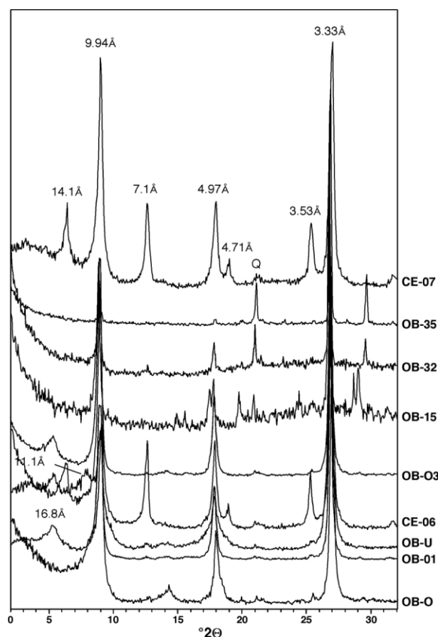
FIGURE 12: Powder X-ray-diffraction of the ethylene glycol-saturated, oriented clay ( <2\ \mu\text{m} ) size fraction of nine K-bentonite beds.
